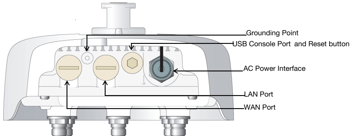
Figure 3 IAP-274 Rear View
