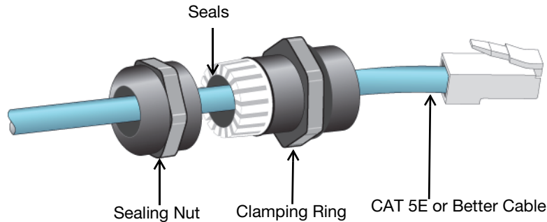
Figure 10 Installing a Cable Gland
