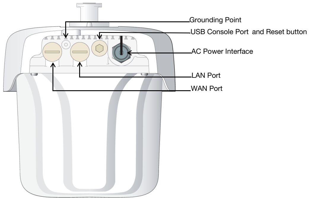
Figure 4 IAP-275 Rear View
