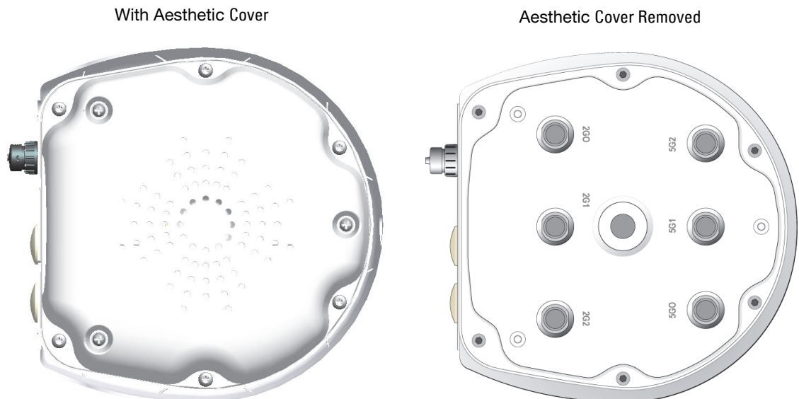
Figure 7 IAP-274 Bottom View
