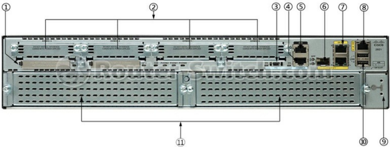
Figure 3 show the expansion slots and ports on the back panel.
